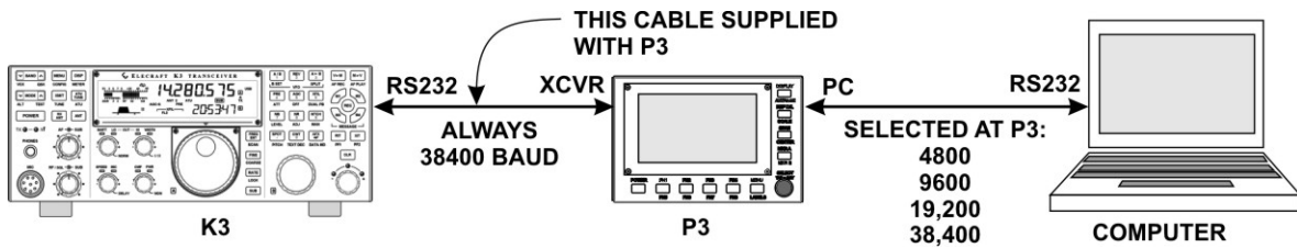
RS232 Communications Path through the P3
